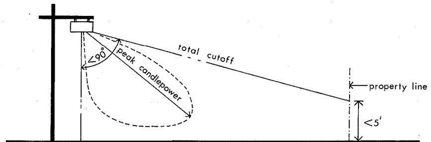
TYPE 3: LUMINAIRE WITH LESS THAN 90^\circ CUTOFF
