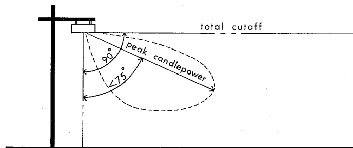
TYPE 2: 90^\circ CUTOFF LUMINAIRE
